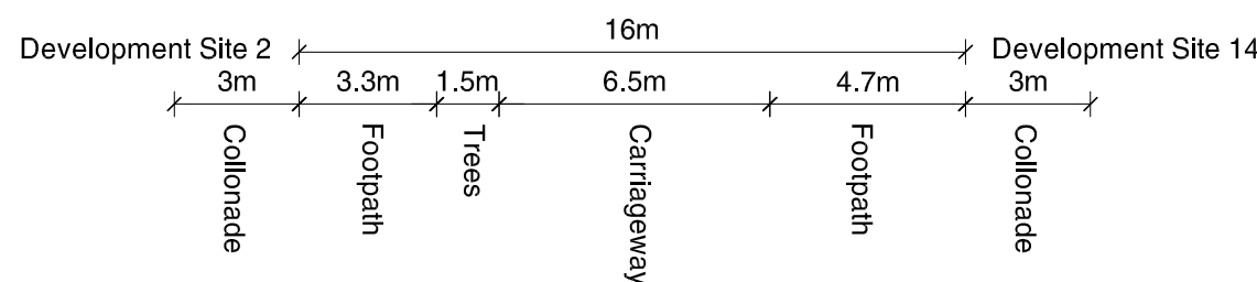
2 DISCOVERY POINT PLACE (NORTH) PART PLAN & SECTION
